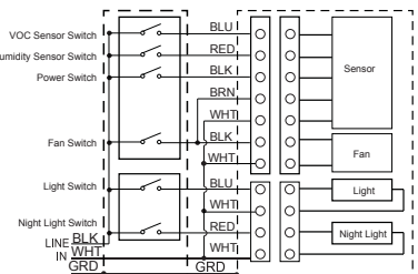
Fan with PCIAQS and PCLK / PCLEDK
