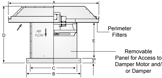
Model HRSB-F Filtered Belt Drive Model HRSD-F Filtered Direct Dive
