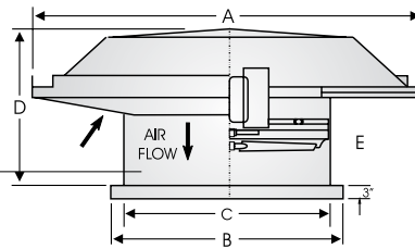
Model HRSB Supply Belt Drive Model HRSD Supply Direct Dive
